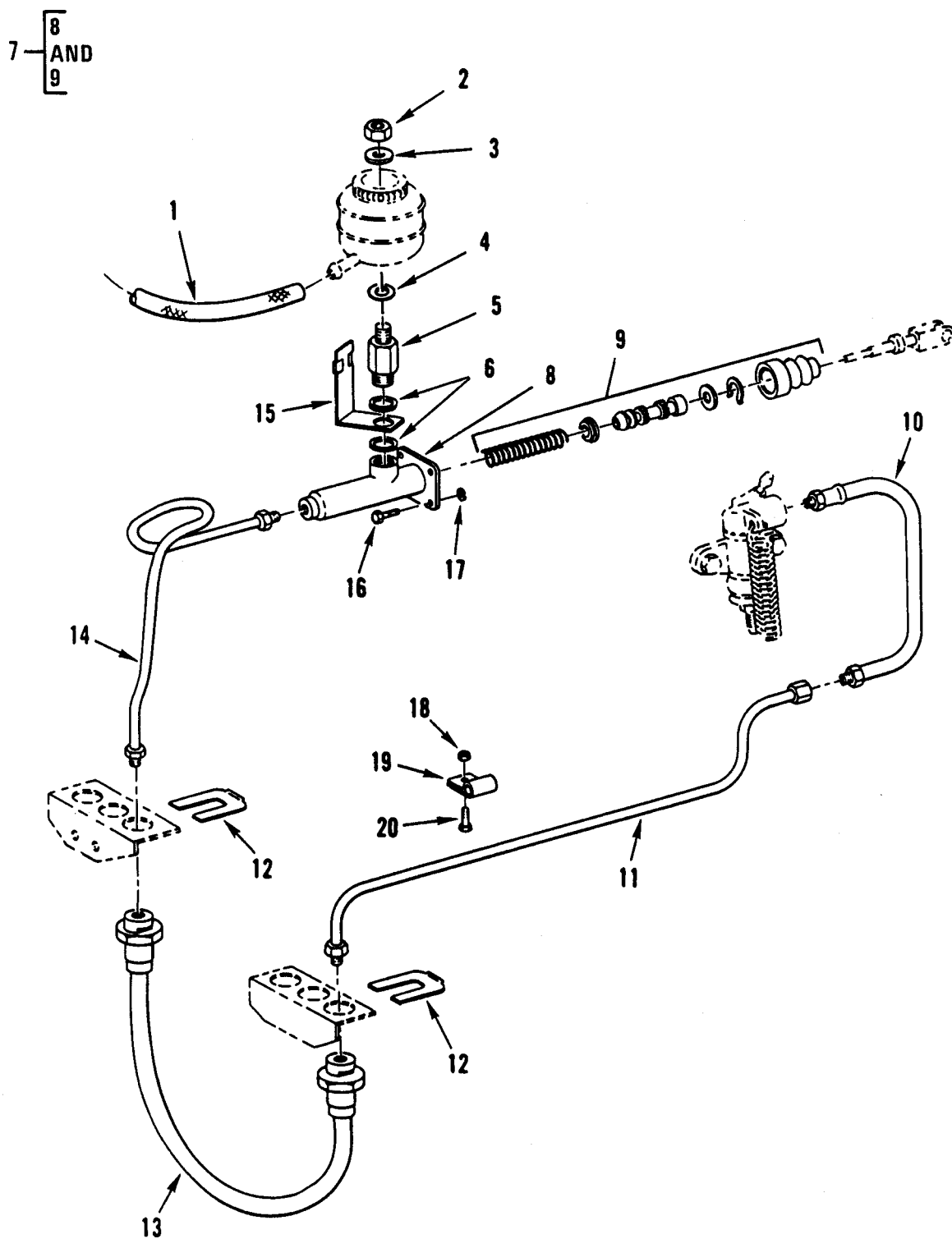
Figure 21. Hydraulic Clutch System – Hydraulic Cylinder Assembly.
