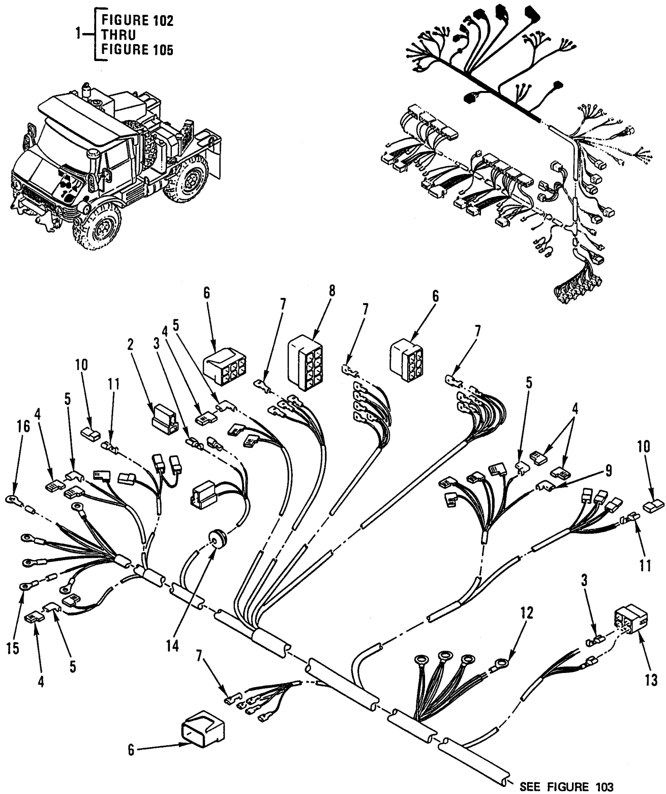
Figure 102. Hull or Chassis Wiring Harness – Main Wiring Harness (Figure 1 of 4).
