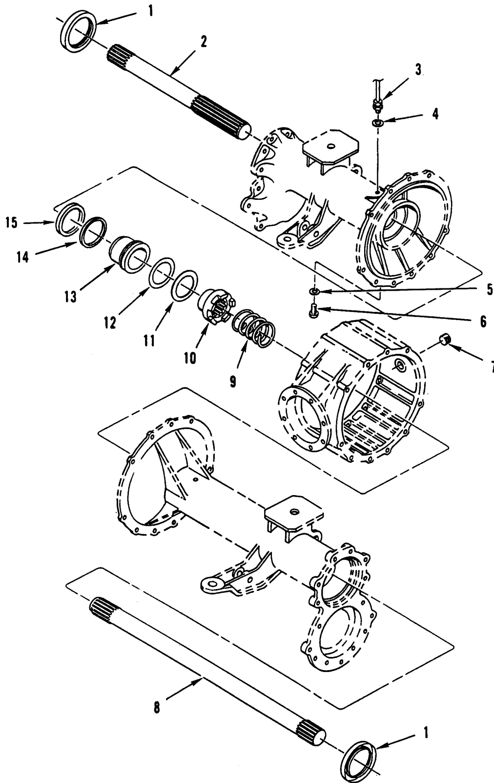
Figure 139. Rear Axle Assembly – Rear Axle.
