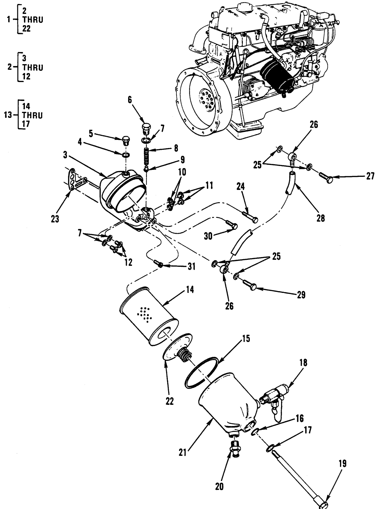
Figure 15. Engine Lubrication System – Fluid Filter, Circulating Valve Cover, and Fluid Filter Element.
