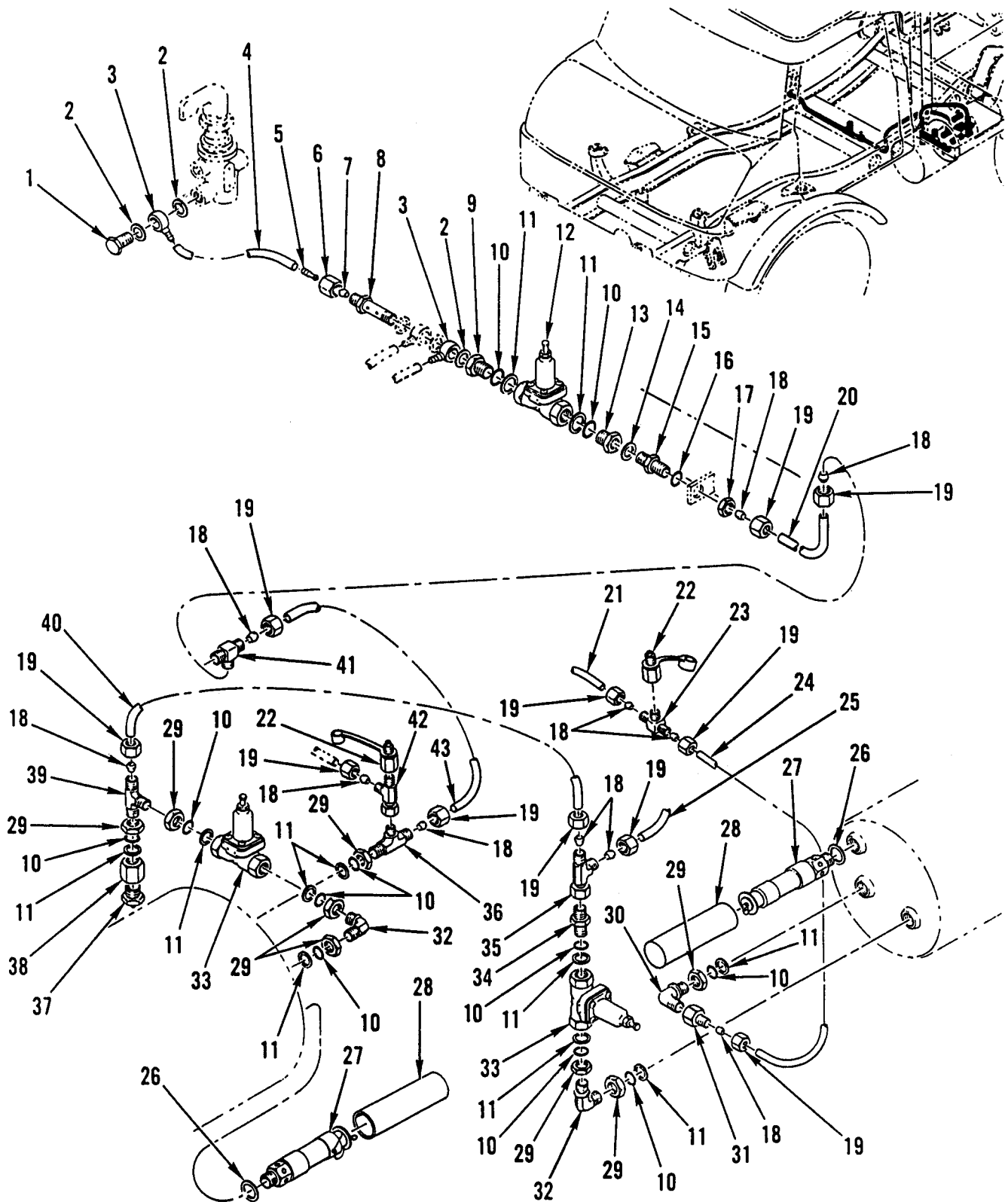
Figure 154. Air Brake System – Air System Valves, Lines, and Fittings.
