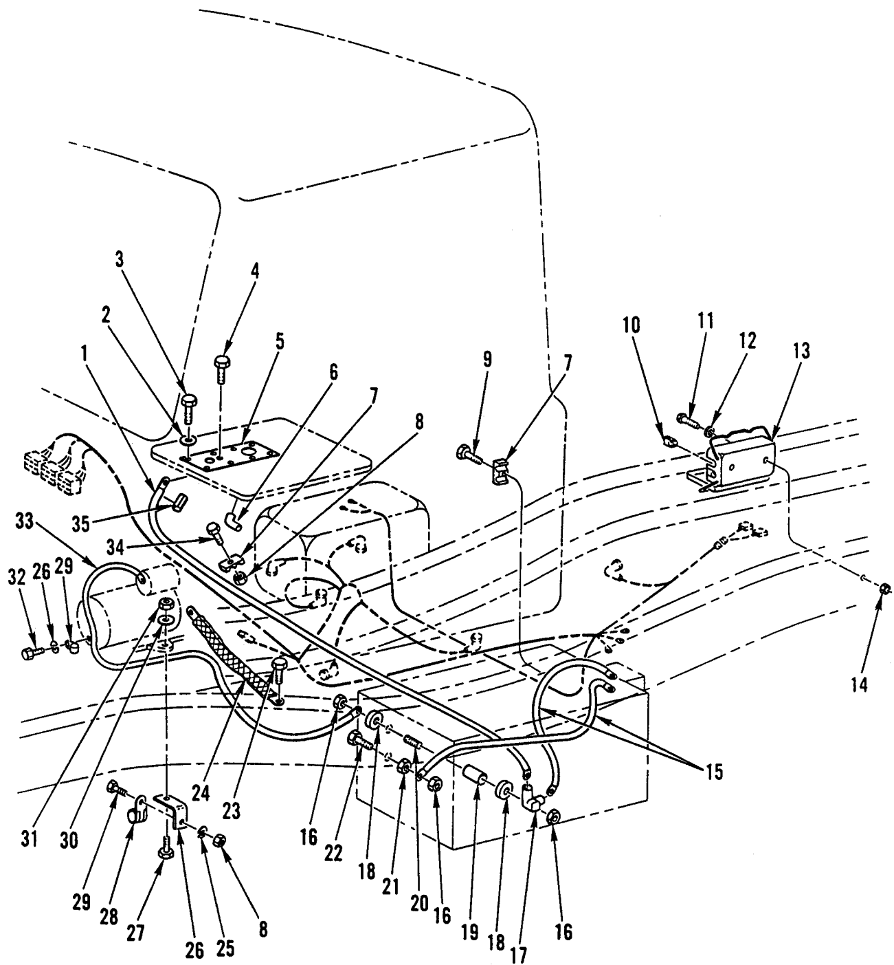
Figure 82. Hull or Chassis Wiring Harness – Electrical Installation (Front Chassis).
